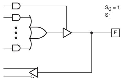
d. Combinatorial/Active-HIGH
