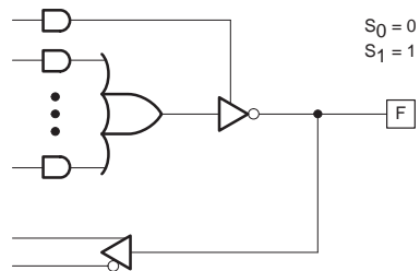
c. Combinatorial/Active-LOW
