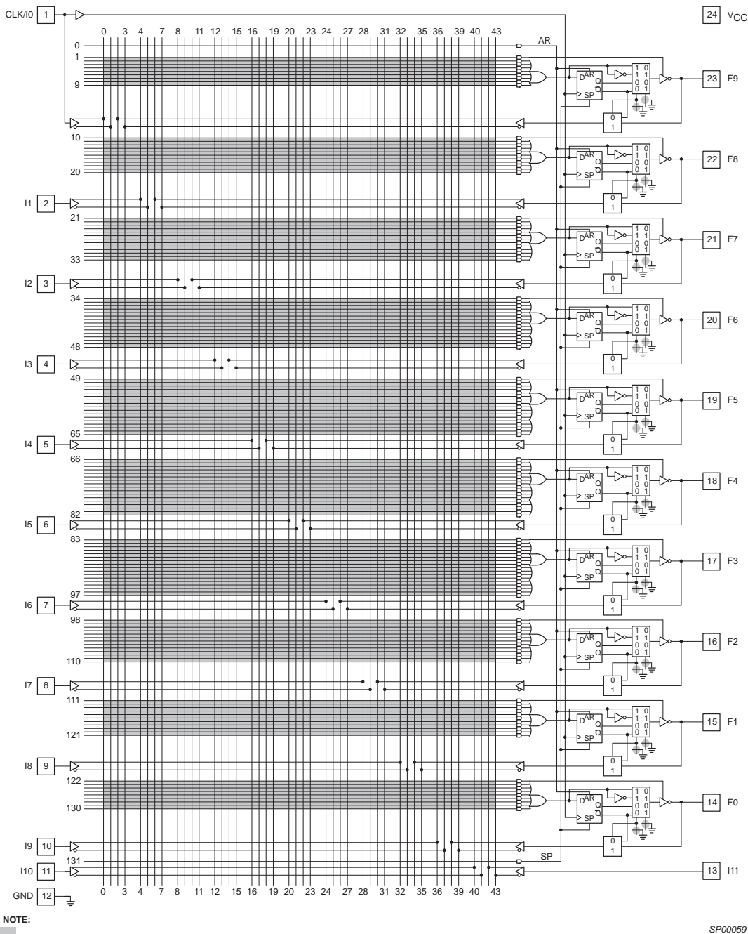
Figure 1: XCR22LV10 Logic Diagram
